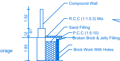
RAIN WATER HARVEST DETAILS
