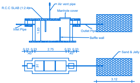
SEPTIC TANK & TRENCH
