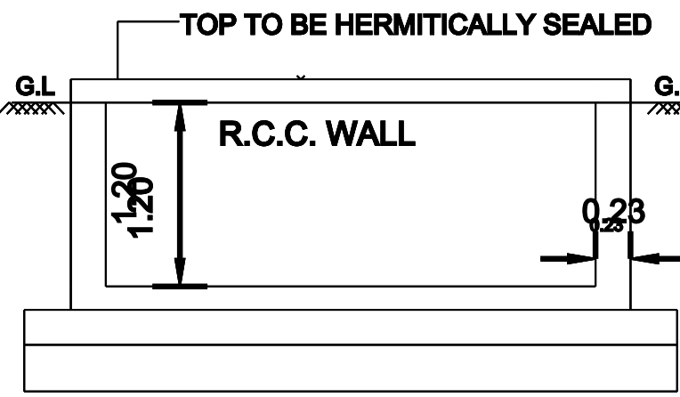
RWH SECTION ( SAMPLE) RWH_CAPACITY_L=2000
