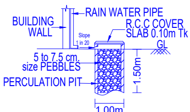
RAIN WATER HARVESTING TRENCH PIT DETAILS
