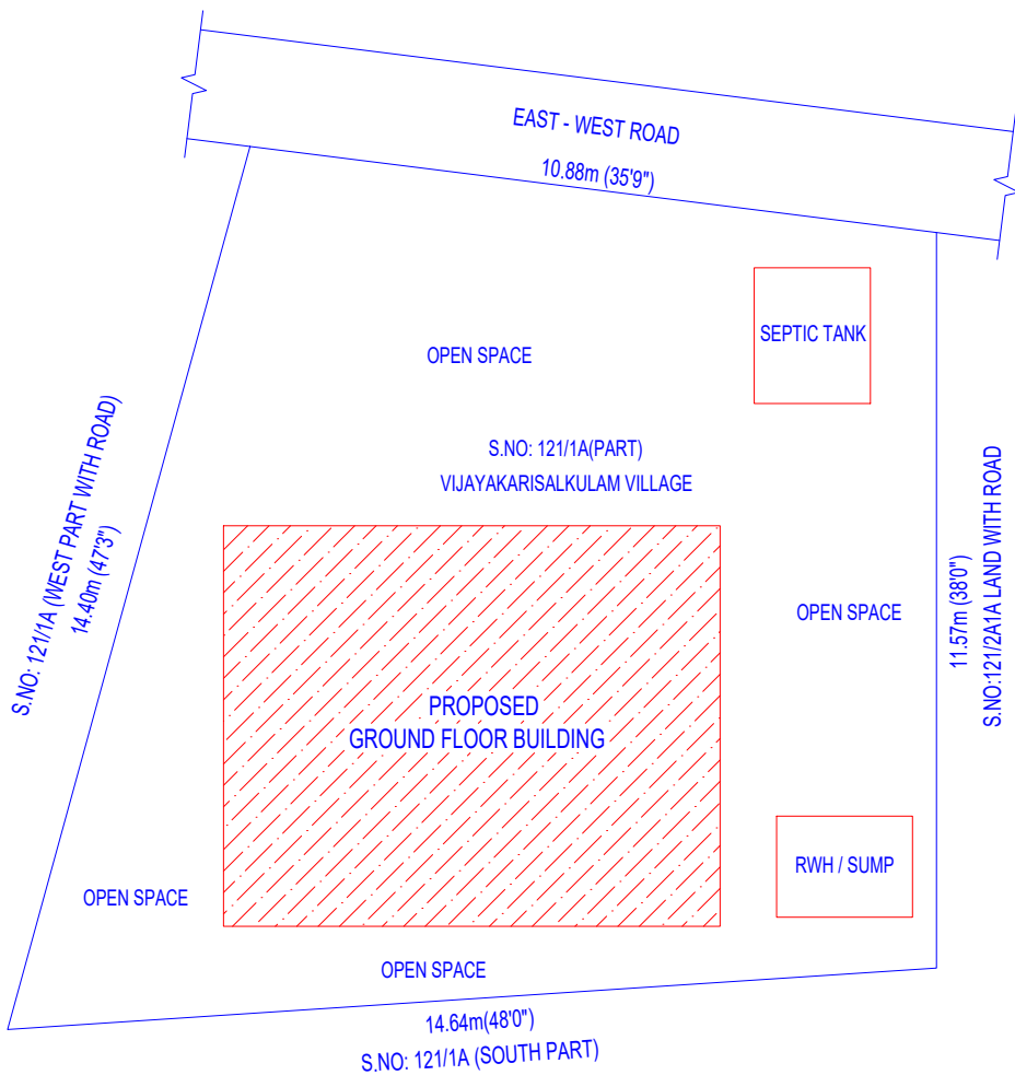
SITE PLAN
