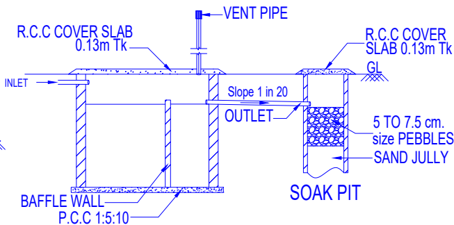
SEPTIC TANK
