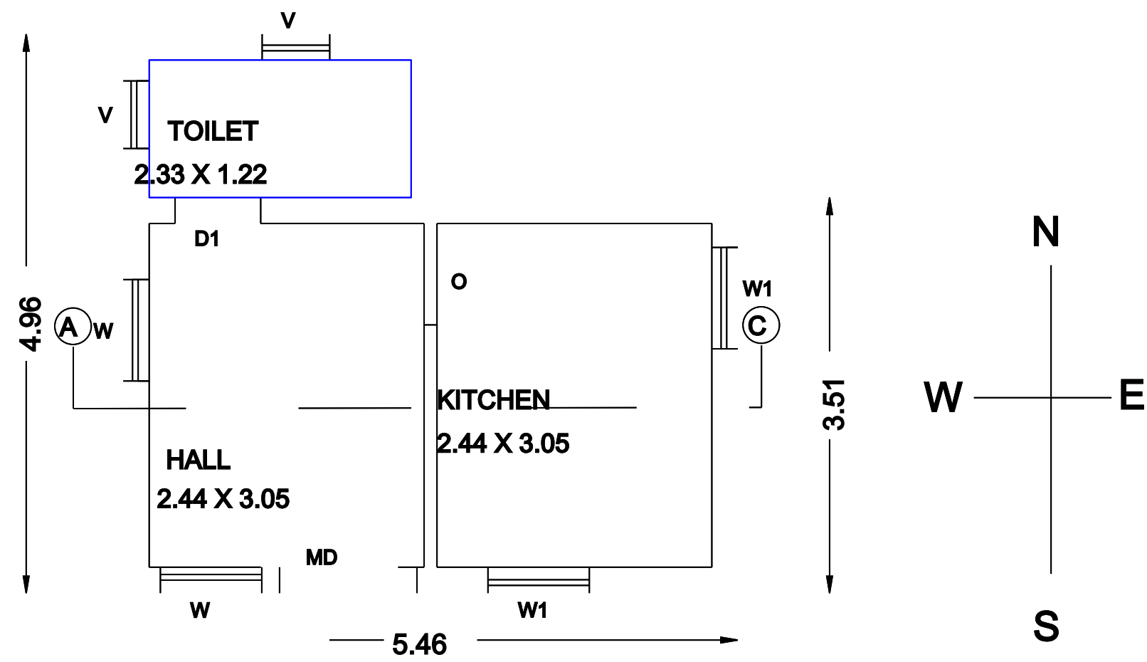
FLOOR PLAN
