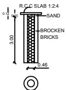
PERCOLATION PIT
