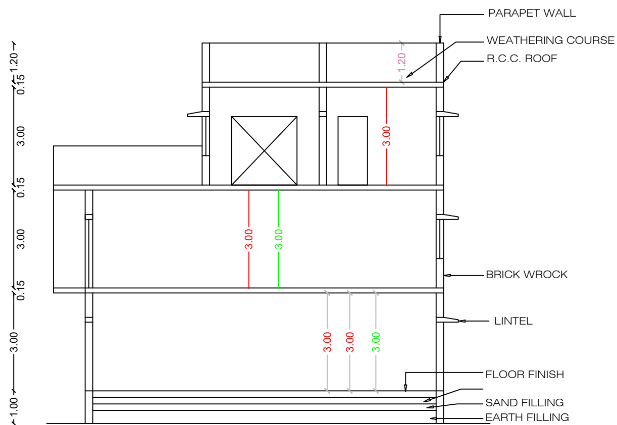
SECTION "XY"
