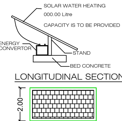
SOLAR SYSTEM
