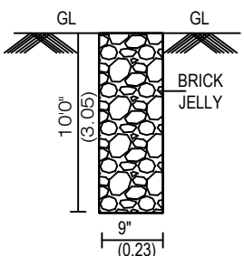
PERCOLATION PIT:-
