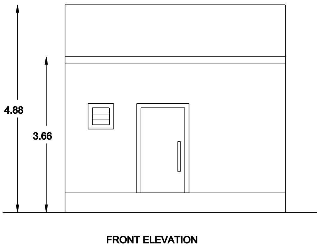
FRONT ELEVATION
