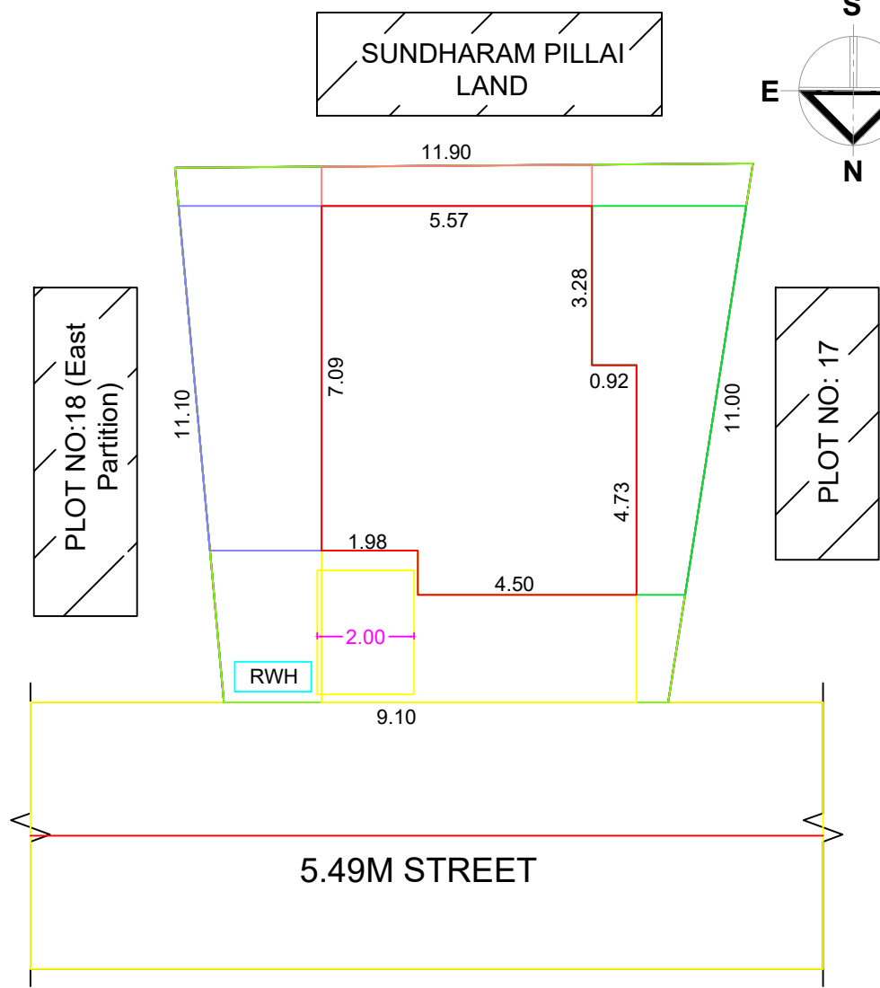
TOPO PLAN Scale 1:100
