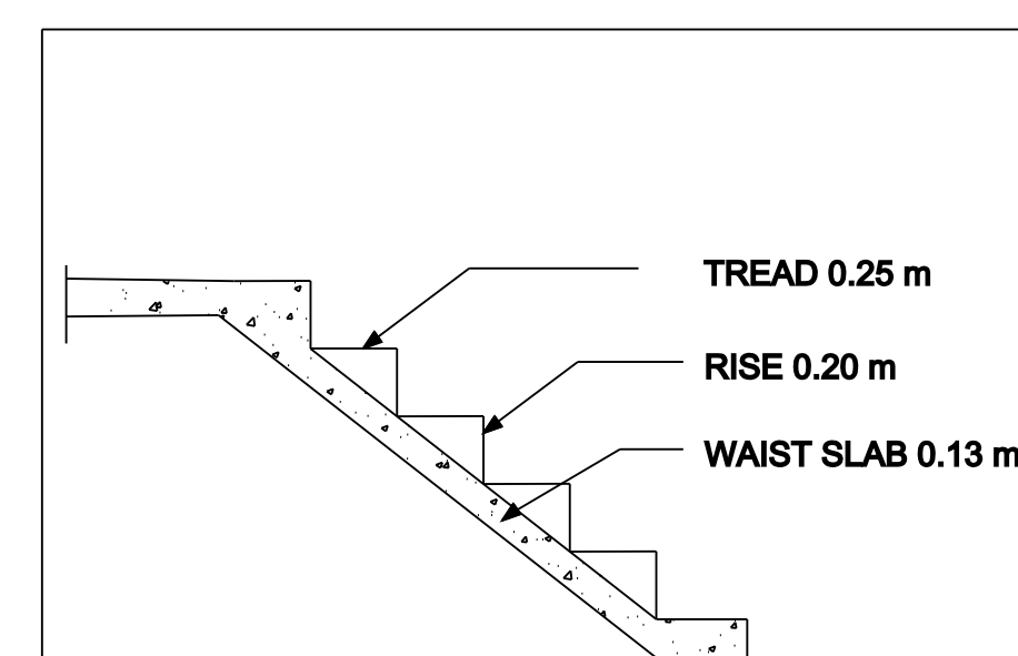
STAIR DETAILS
