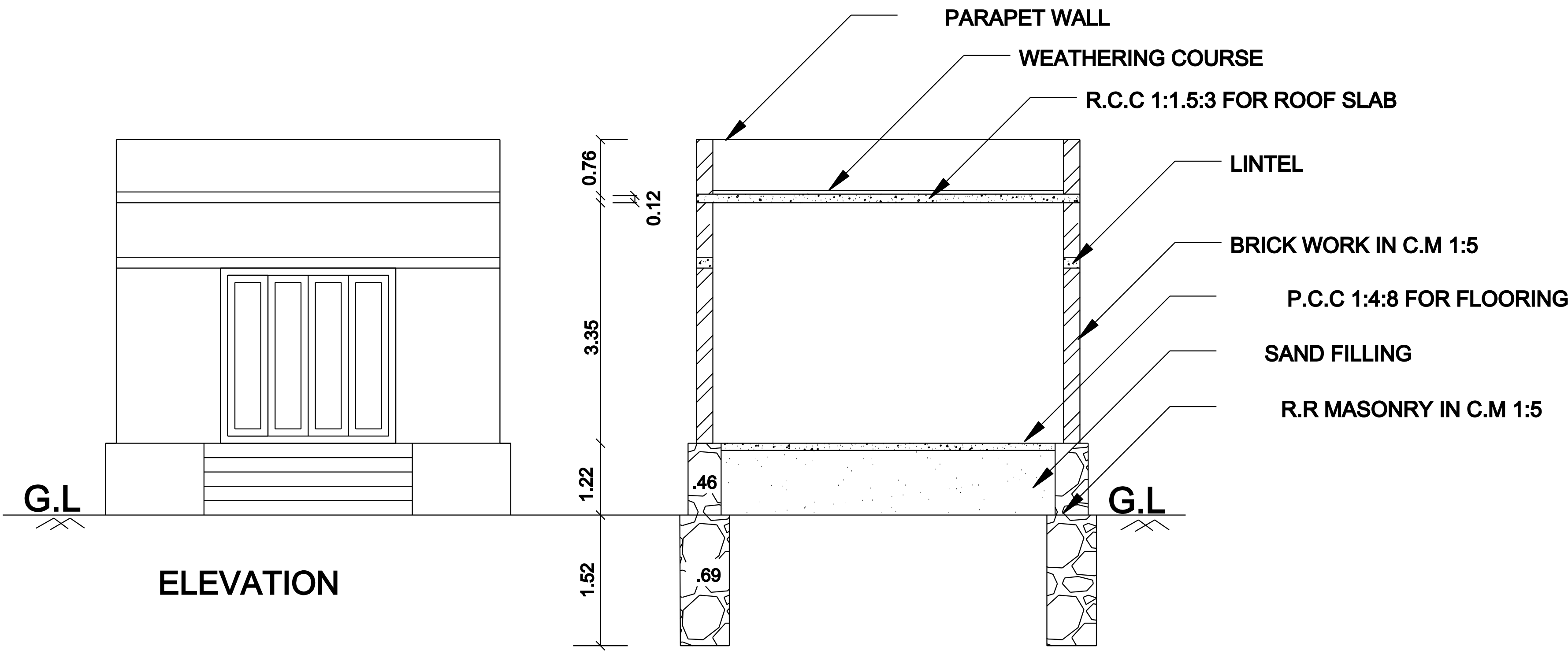
SECTION ON "DC"
