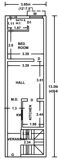
GROUND FLOOR PLAN
