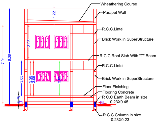
SECTION ON "PQ" SCALE 1:100
