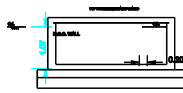
RWI SECTION (SAMPLE)
