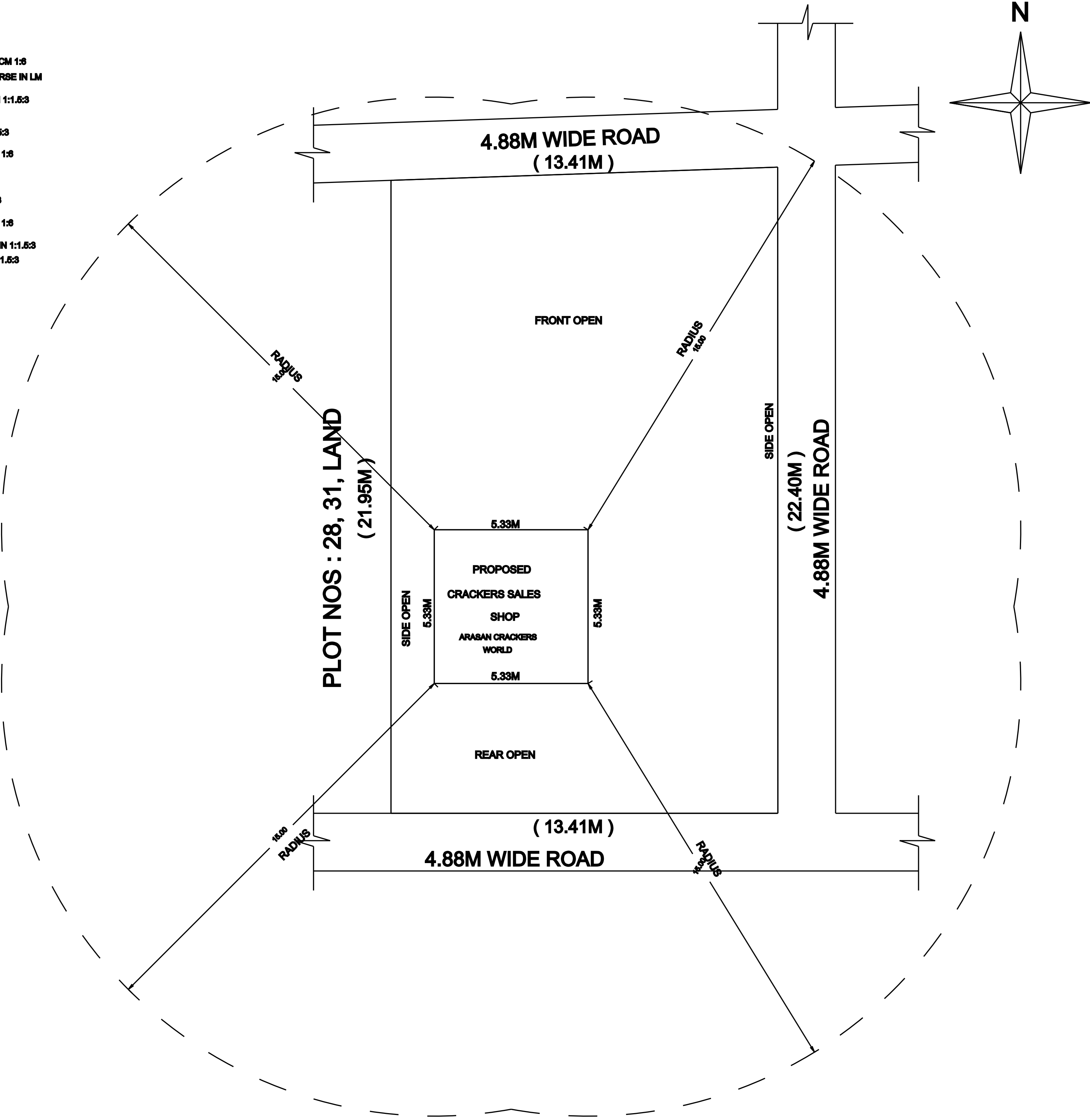
SITE PLAN
