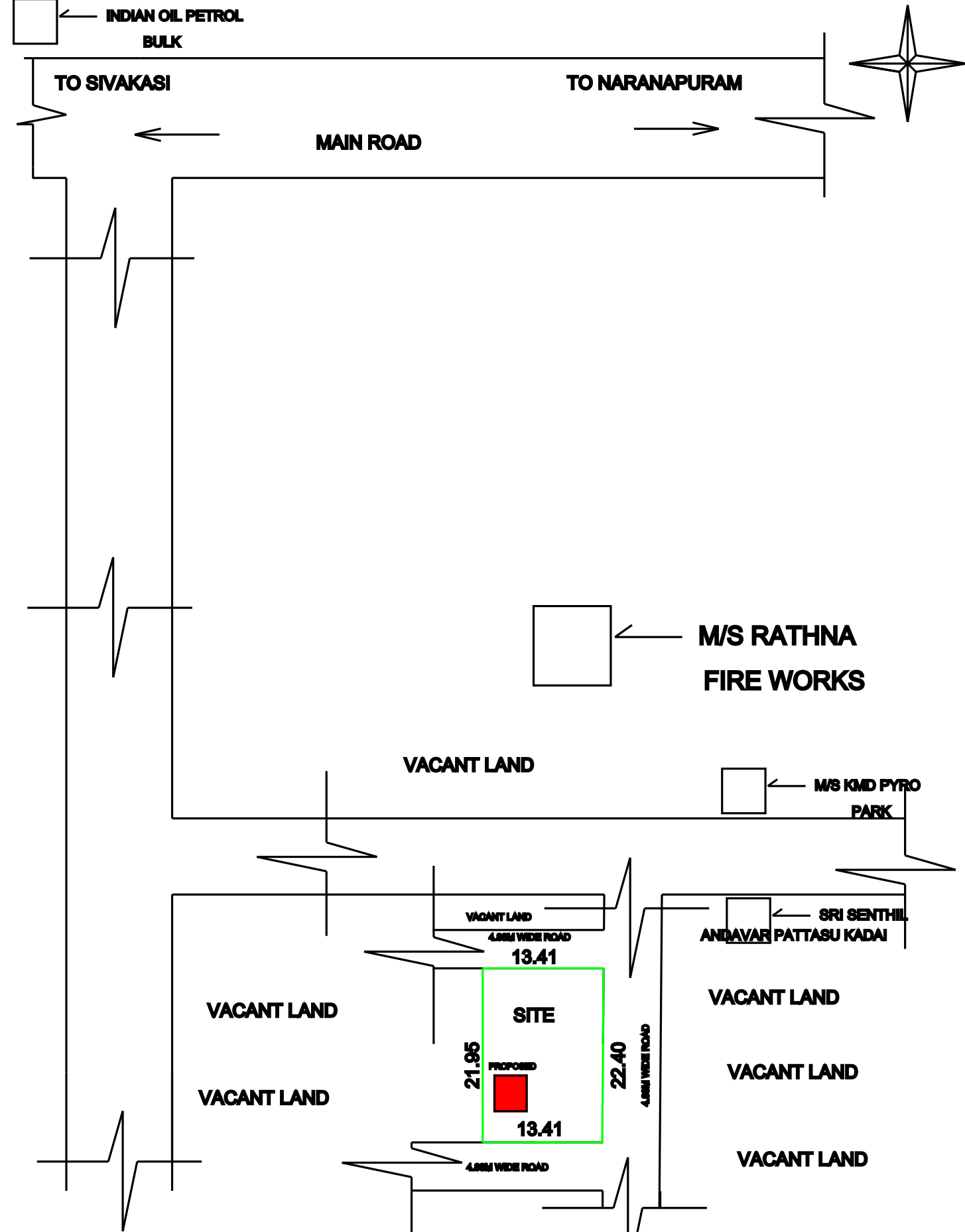
KEY PLAN
