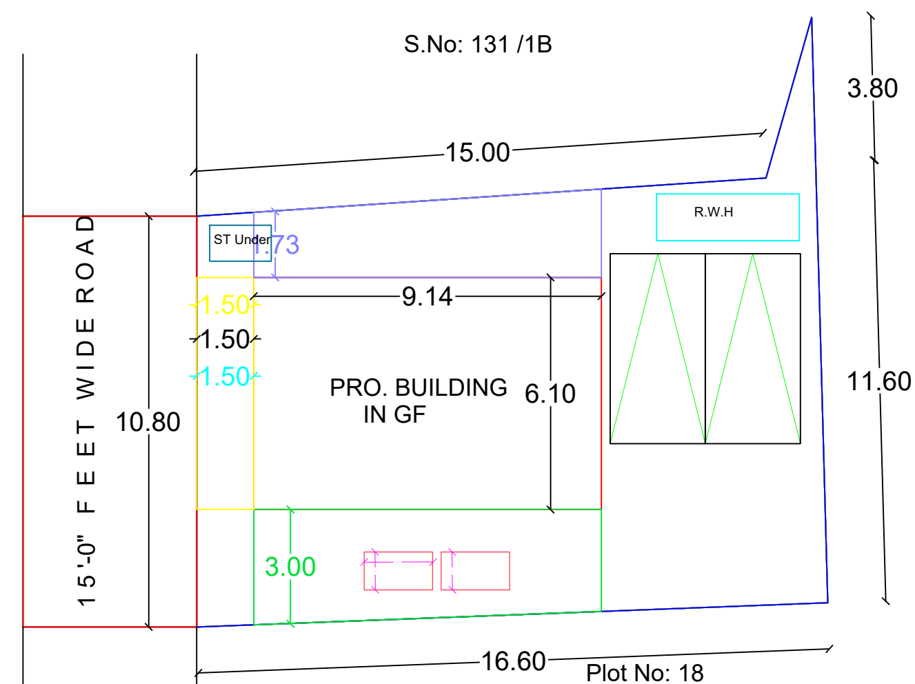
SITE PLAN
