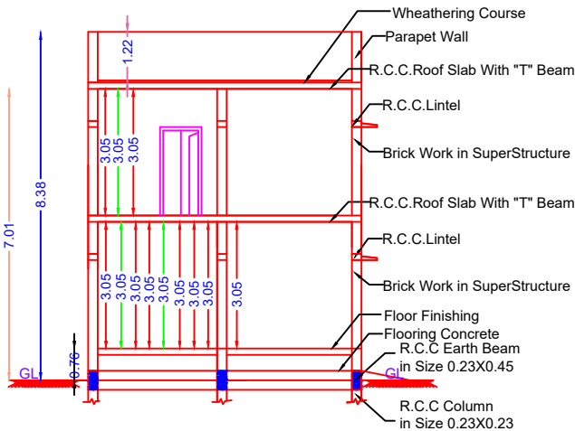
SECTION ON "PQ" (SCALE 1:100)
