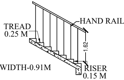
STAIRCASE DETAILS
