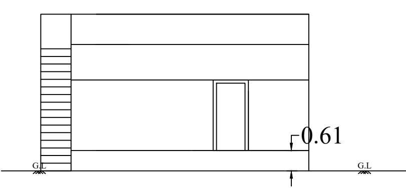
FRONT ELEVATION
