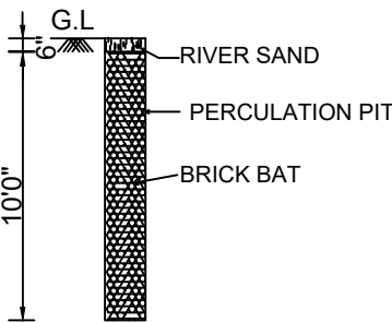
PERCOLATION PIT
