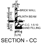
SECTION - CC
