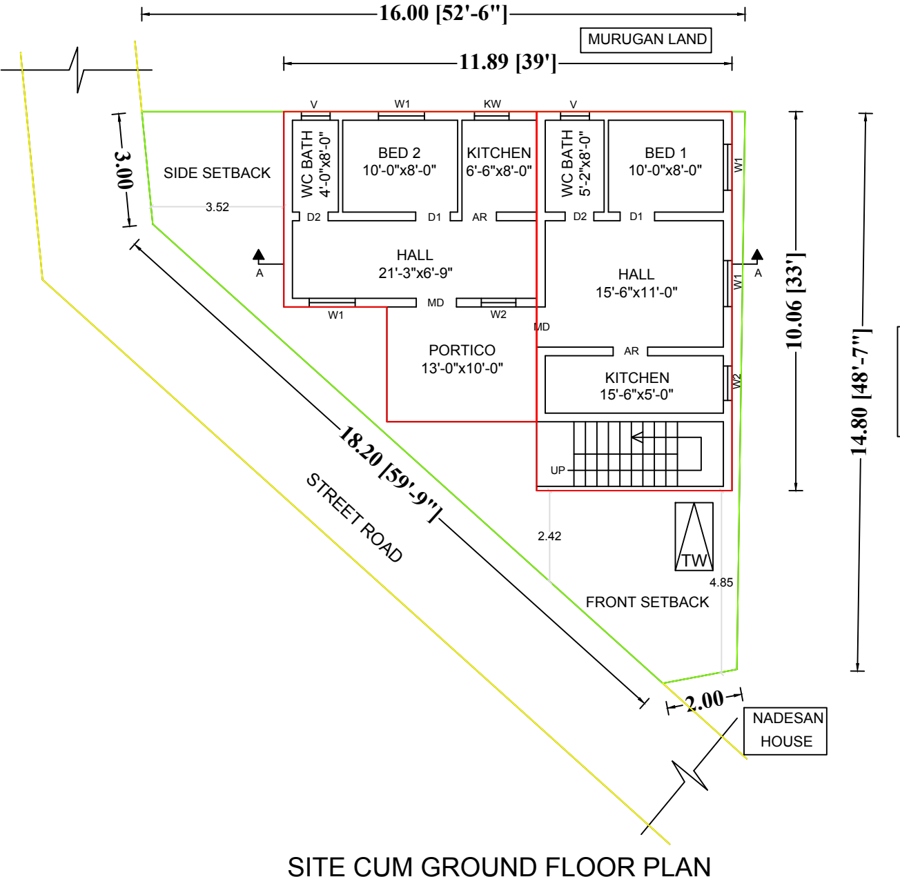
SITE CUM GROUND FLOOR PLAN
