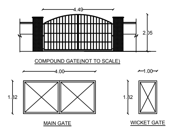
MAIN GATE
