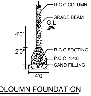
COLOUMN FOUNDATION
