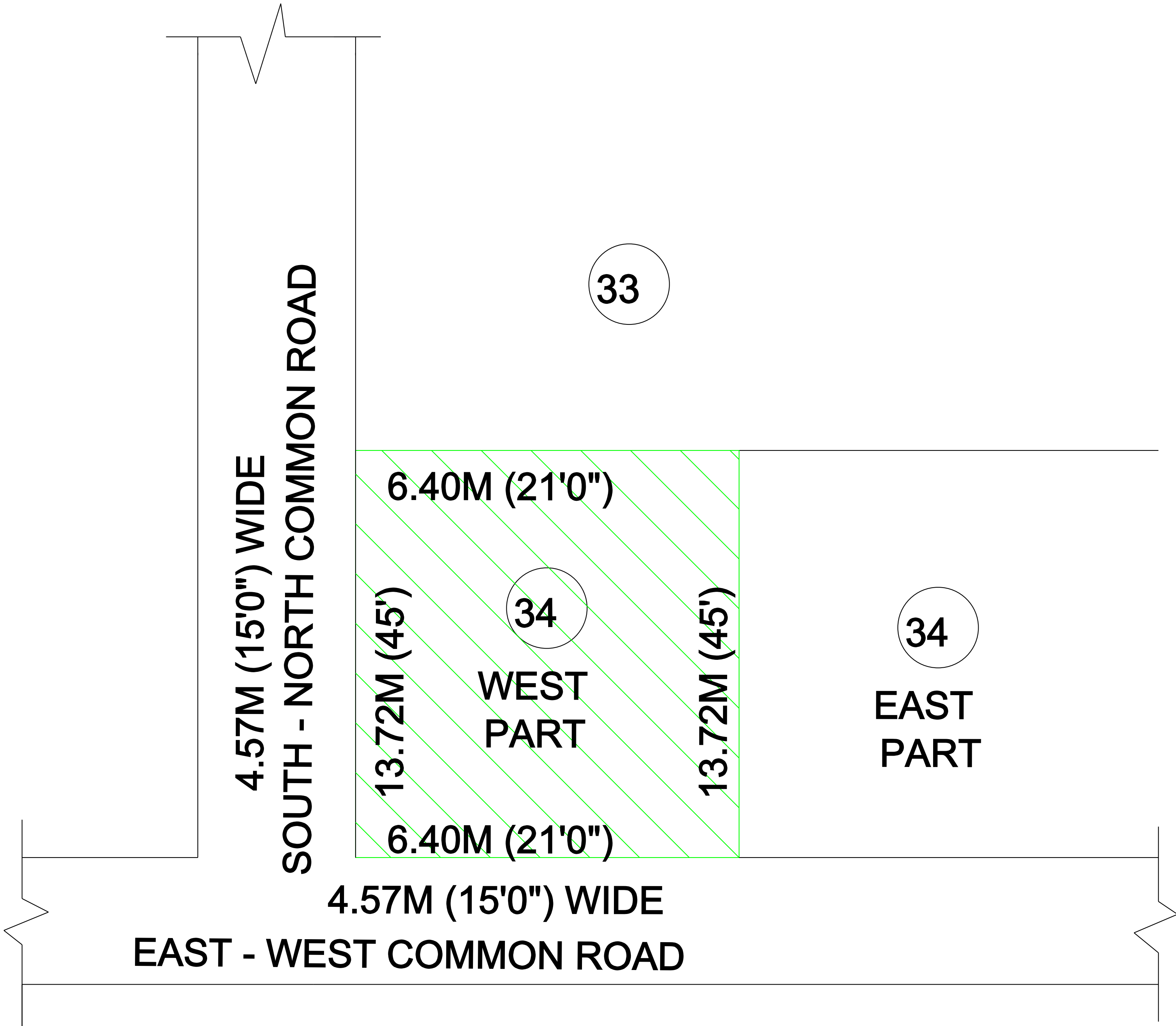
LOCATION PLAN
