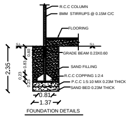
FOUNDATION DETAILS
