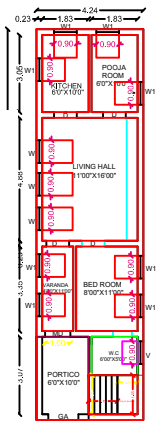
PROPOSED GROUND FLOOR
