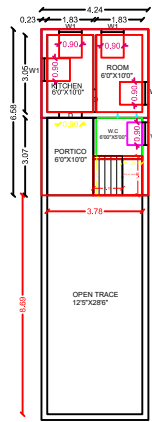
PROPOSED FIRST FLOOR
