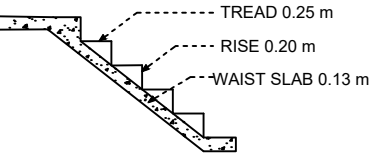
STAIR DETAILS
