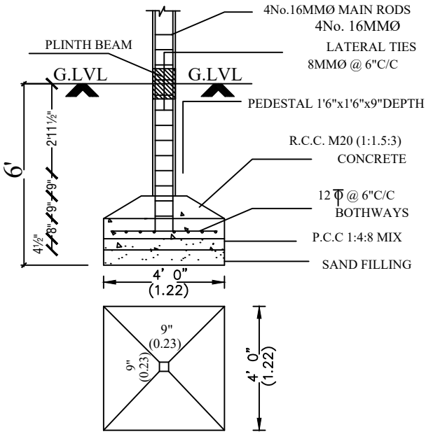
FOUNDATION DETAIL [SCALE: 1:50]
