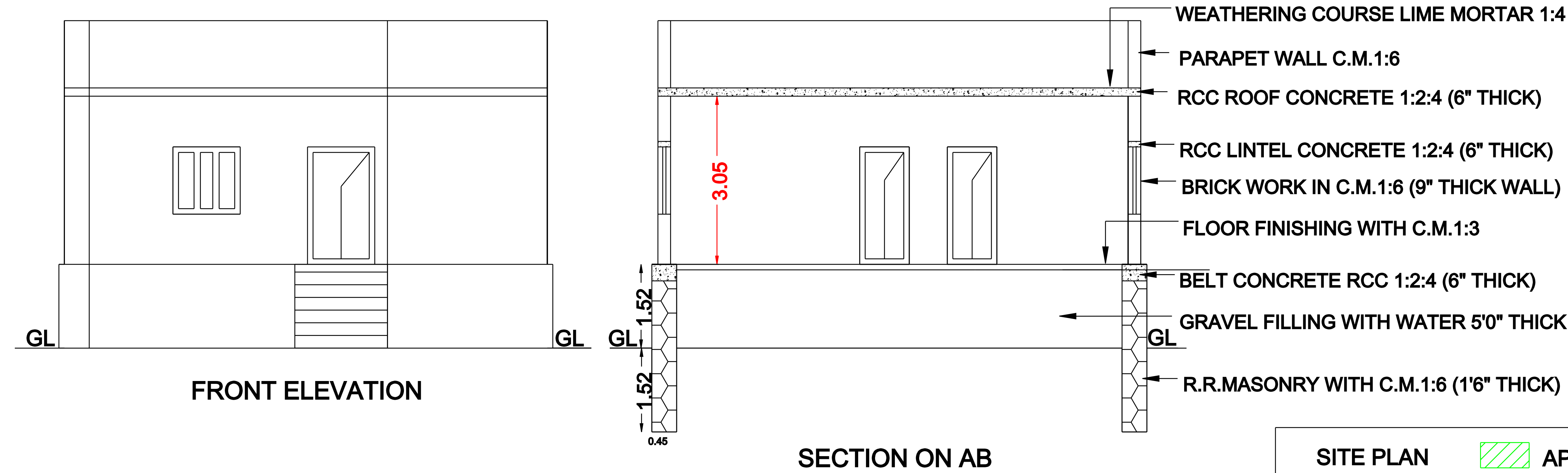
SECTION ON AB
