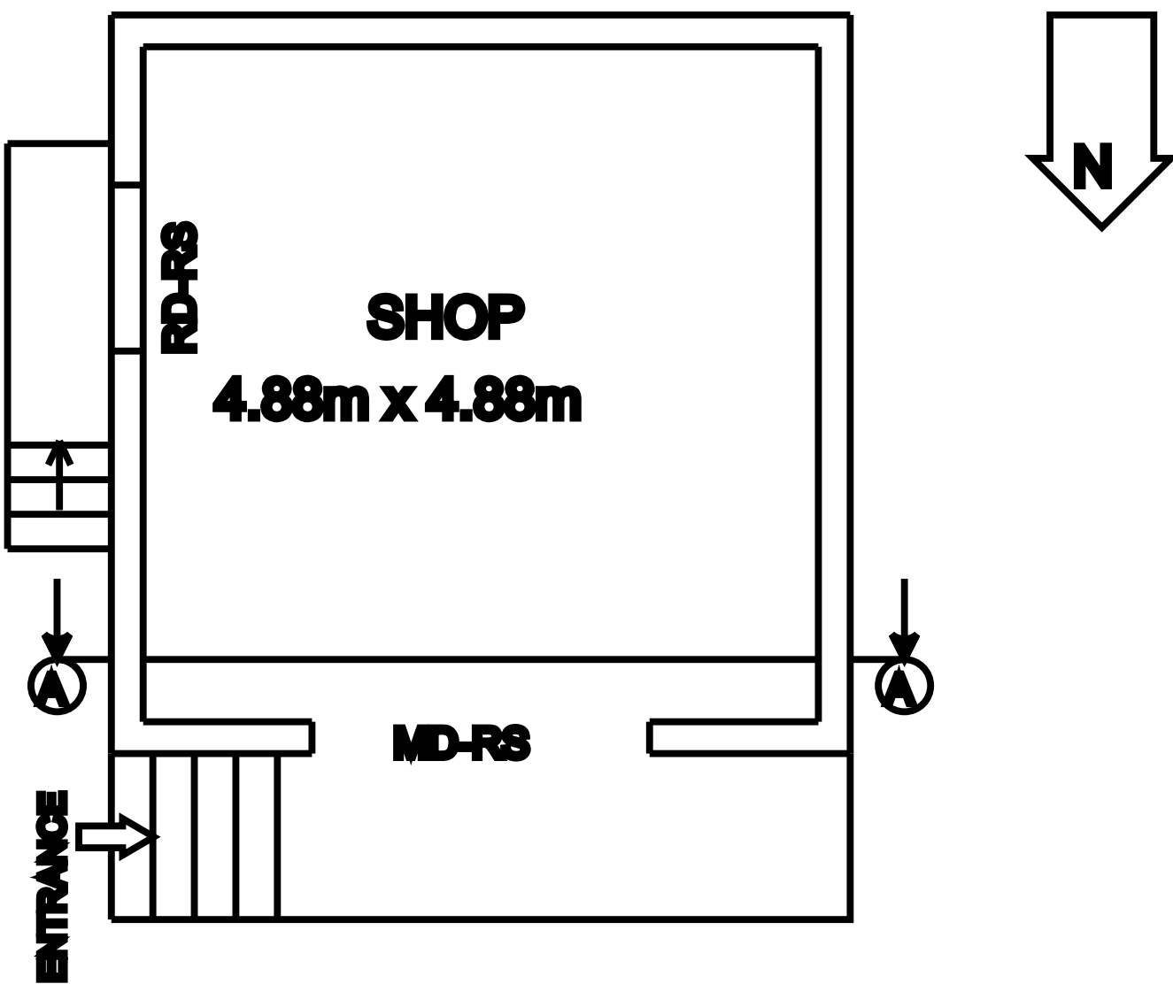
FLOOR PLAN
