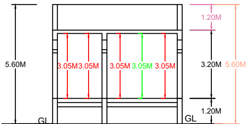
SECTION AB
