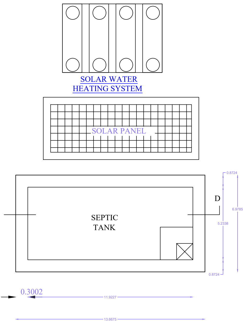
PLAN OF SEPTIC TANK SCALE 1"=2'-0"
