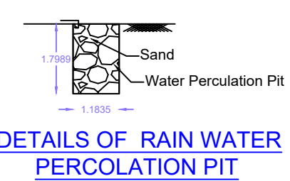
DETAILS OF RAIN WATER PERCOLATION PIT (SCALE 1:100)
