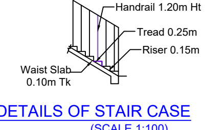
DETAILS OF STAIR CASE (SCALE 1:100)
