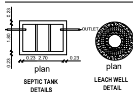
SEPTIC TANK DETAILS
