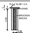
PERCOLATION PIT
