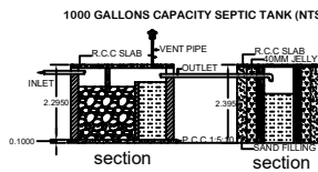
1000 GALLONS CAPACITY SEPTIC TANK (NTS)
