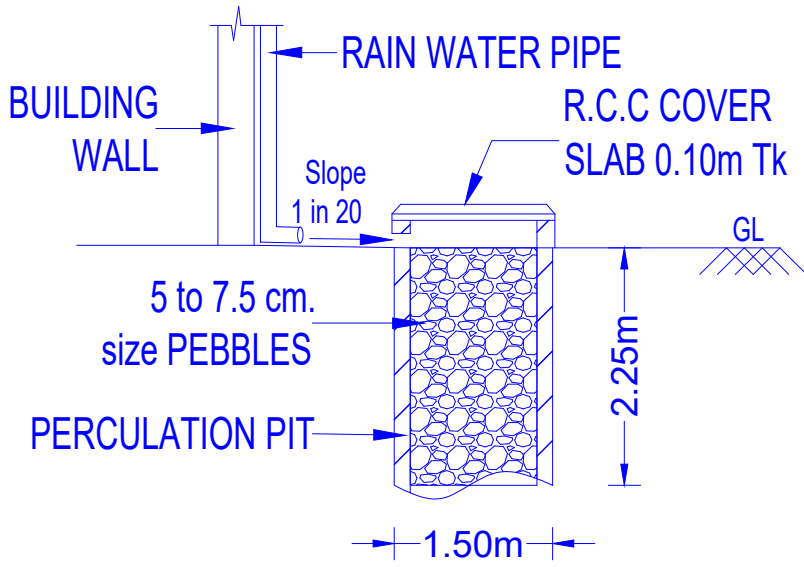
RAIN WATER HARVESTING TRENCH PIT DETAILS
