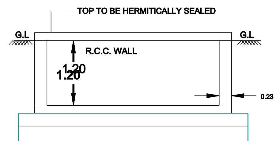
RWH SECTION
