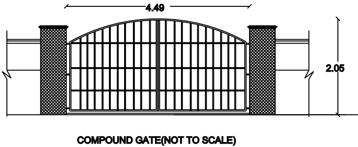
COMPOUND GATE(NOT TO SCALE)
