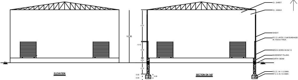
SECTION ON 'AB'
