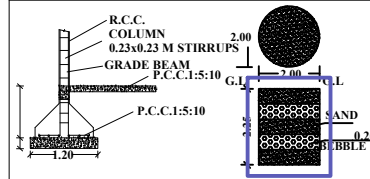
COLUMN DETAIL
