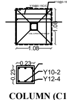
COLUMN (C1)
