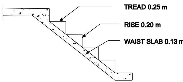
STAIR DETAILS
