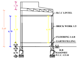
"SECTION "AB"
