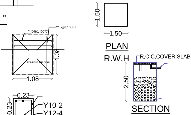
COLUMN (C1)
