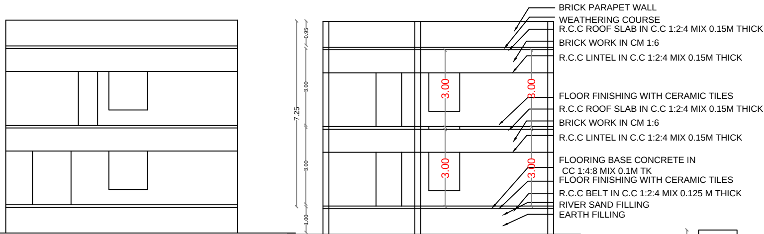
FRONT ELEVATION
