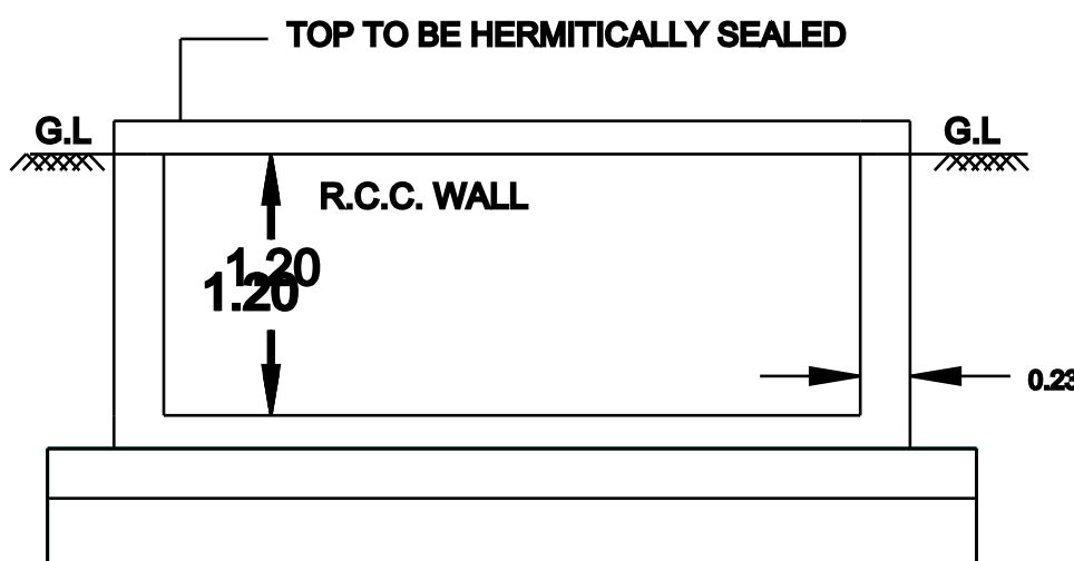
RW SECTION
