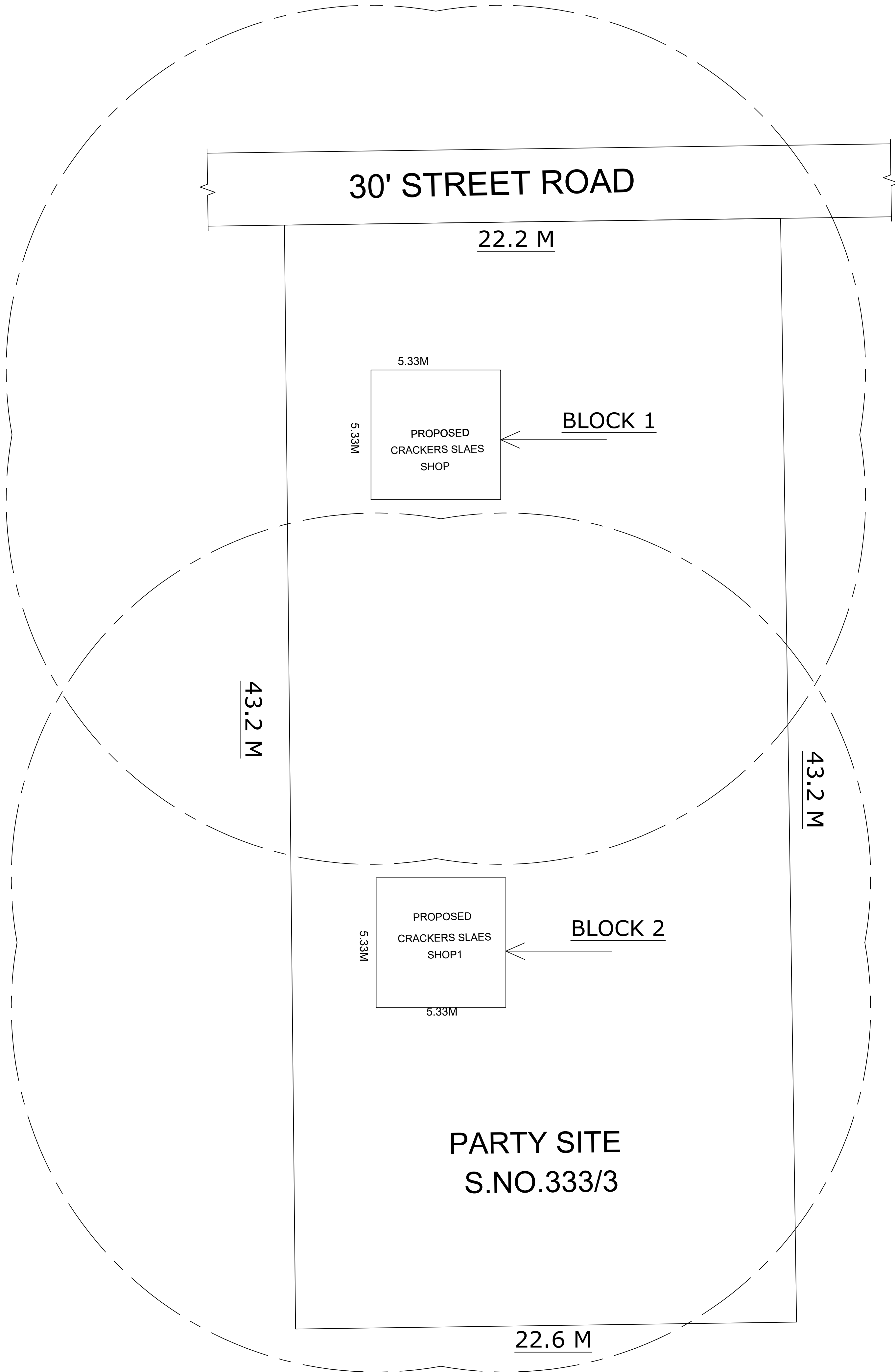
SITE PLAN
