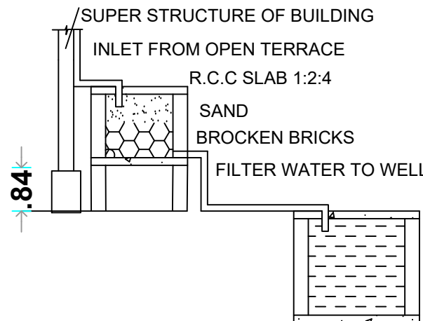
RAINWATER HARVESTING
