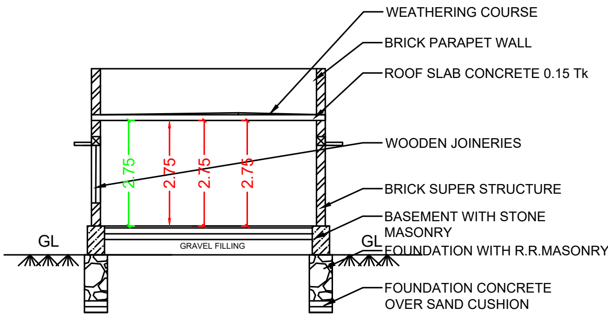
SECTION VIEW"AA"
