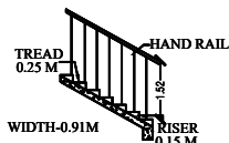
STAIRCASE DETAILS
