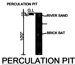
PERCOLATION PIT
