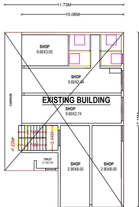
EXIST.GROUND FLOOR PLAN
