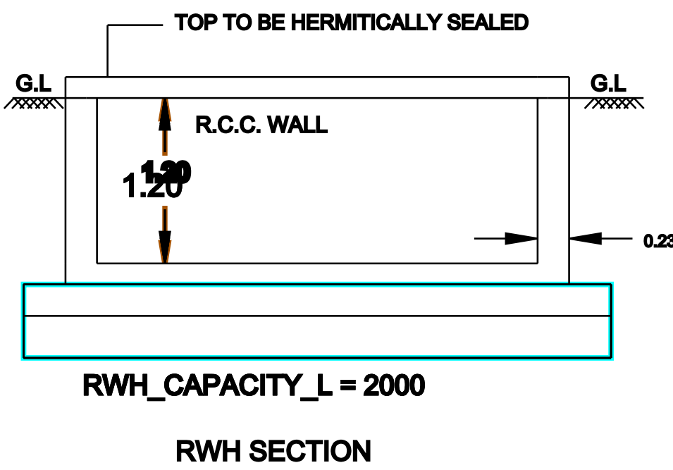
RWH SECTION
