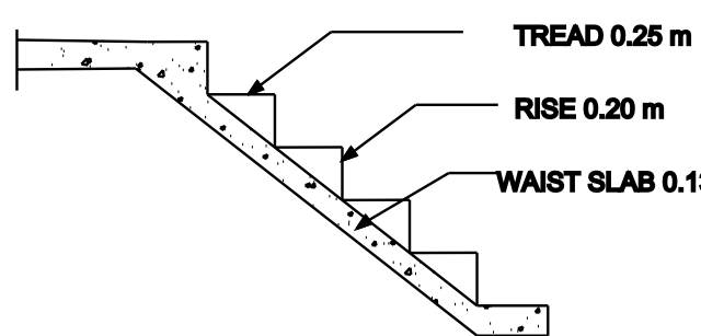
STAIR DETAILS
