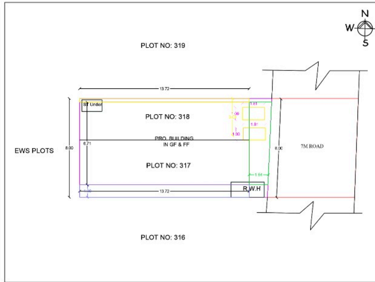
SITE PLAN
