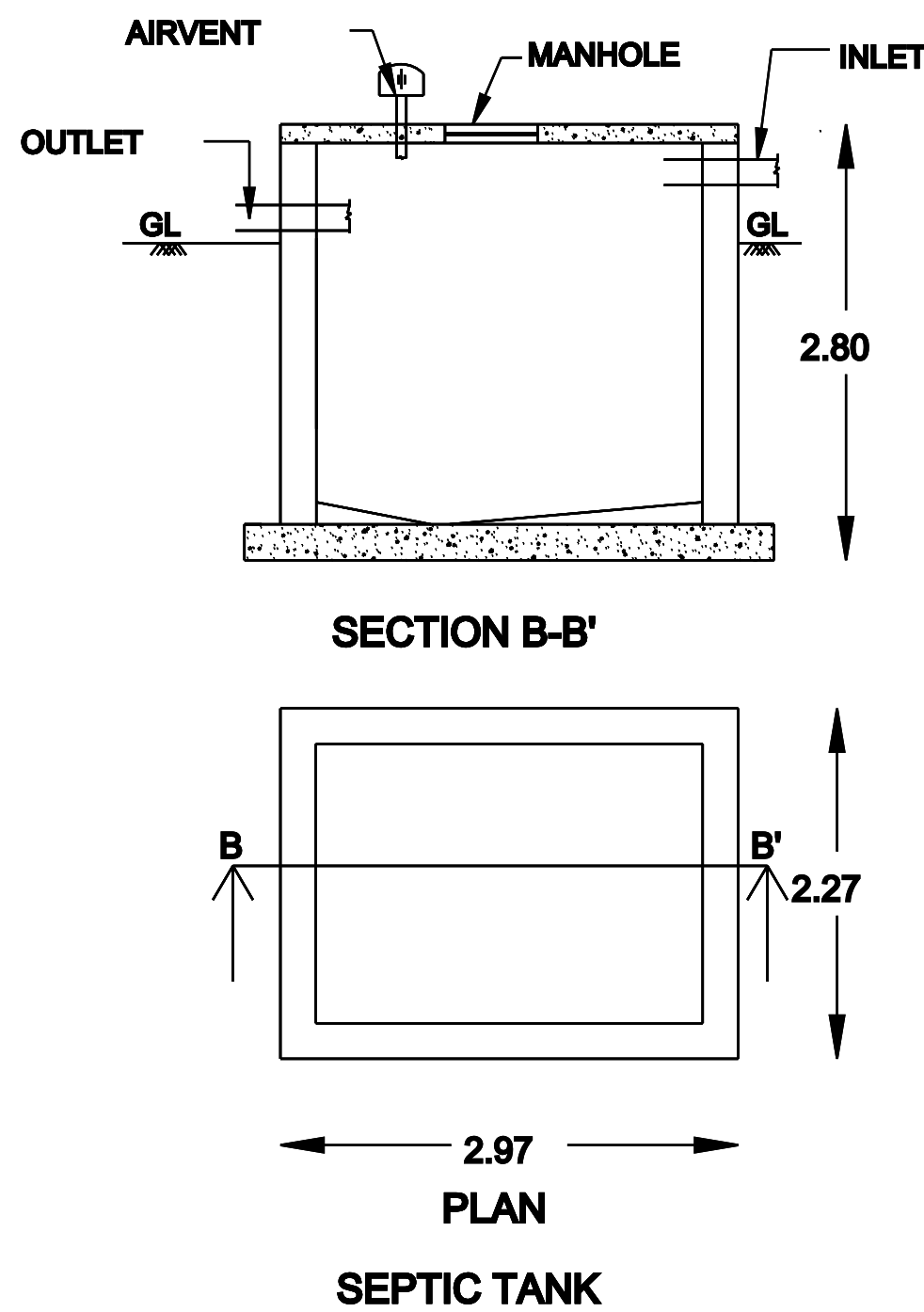
SEPTIC TANK
