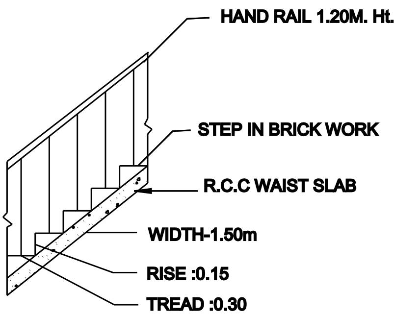
STAIR DETAIL
