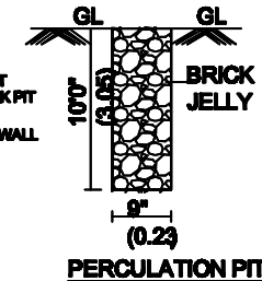
PERCOLATION PIT
