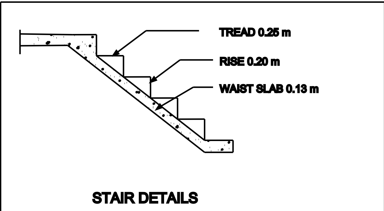
STAIR DETAILS
